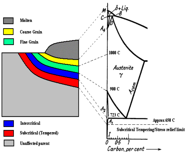
Figure 1. Iron-carbon phase diagram showing the transition points relating to a weld HAZ (Reference 6)
